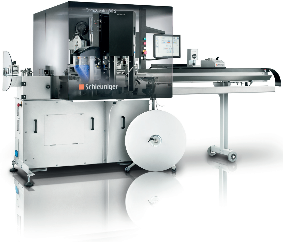
CrimpCenter 36 S Fully Automatic Crimping Machine
